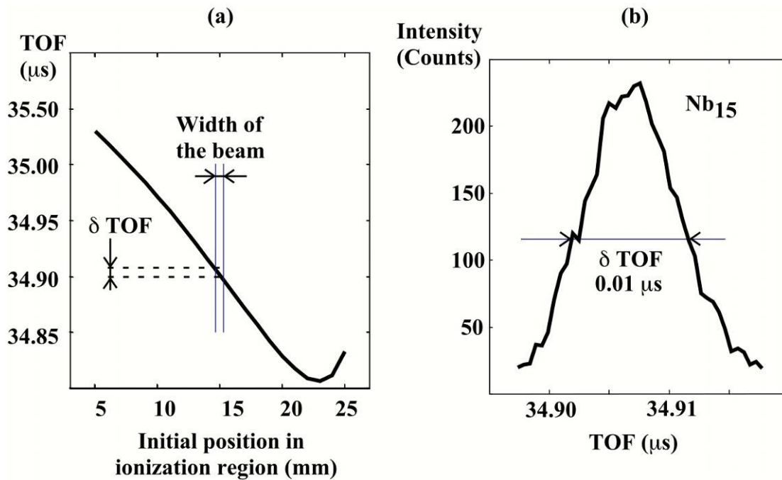
Figure 16: Position sensitive mode of the mass spectrometer. (a) Time of flight (TOF) in microseconds for a \text{Nb}_{15} cluster as a function of the initial position in the ionization region. (b) Peak profile of \text{Nb}_{15} as a function of time of flight. The time resolution of this peak is 3500, and mass resolution 1750.
