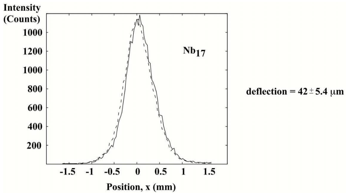
Figure 18: Position-Sensitive mass spectrum with and without electric field for Nb 17 at 300 K. Dashed line is with field off. Continuous line is with E= 80 kV/cm.
