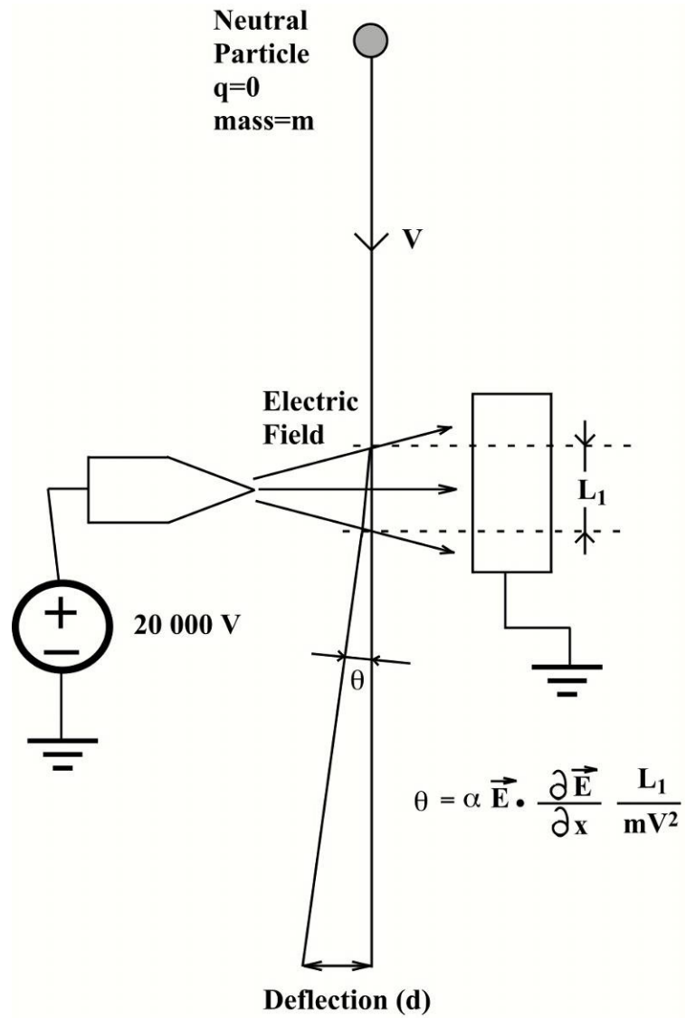
Figure 1: Principle of the electric deflection experiment. A neutral particle passes through a region of inhomogeneous electric field where it changes its trajectory producing a deflection, which is measured.
