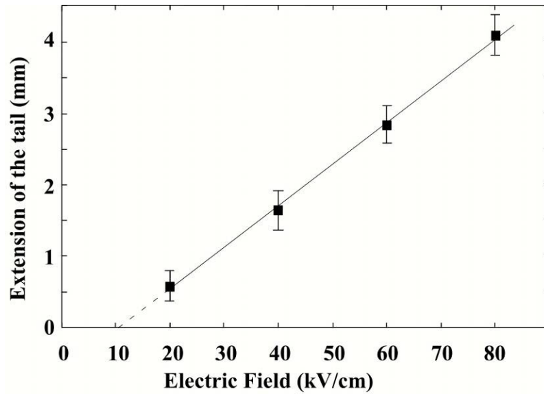
Figure 23: Extension of the observed tail for Nb 14 as a function of electric field at 50 K. The straight line is a linear fit to the data which extrapolates to give an intercept of 11 kV/cm, which is interpreted as the electric field needed to uncouple the dipole moment.
