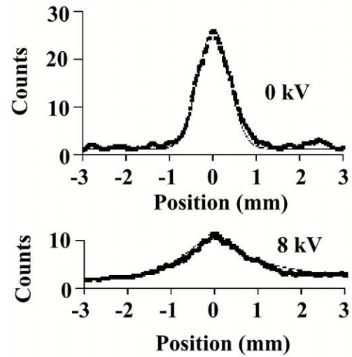
Figure 28: The model by P. Dugourd [P. Dugourd, 2001] correctly predicts the shape of the deflected peak of a molecule of Ti C 60 with a dipole of 8.1 D. Filled squares are experimental values, thin dashed line their model prediction. The experiment at 8 kV is done with an electric field of 48.3 kV/cm.
