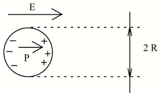
Figure 2: A classical perfect spherical conductor is polarized by an electric field. The induced dipole moment is parallel to the electric field.
