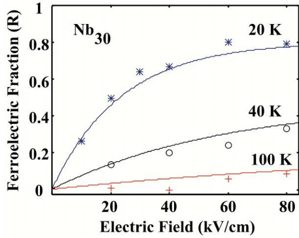
Figure 30: Ferroelectric fraction (R) experimentally measured at 3 temperatures and several electric field intensities for Nb 30 . The continuous lines are the fitting functions calculated in the proposed model.
