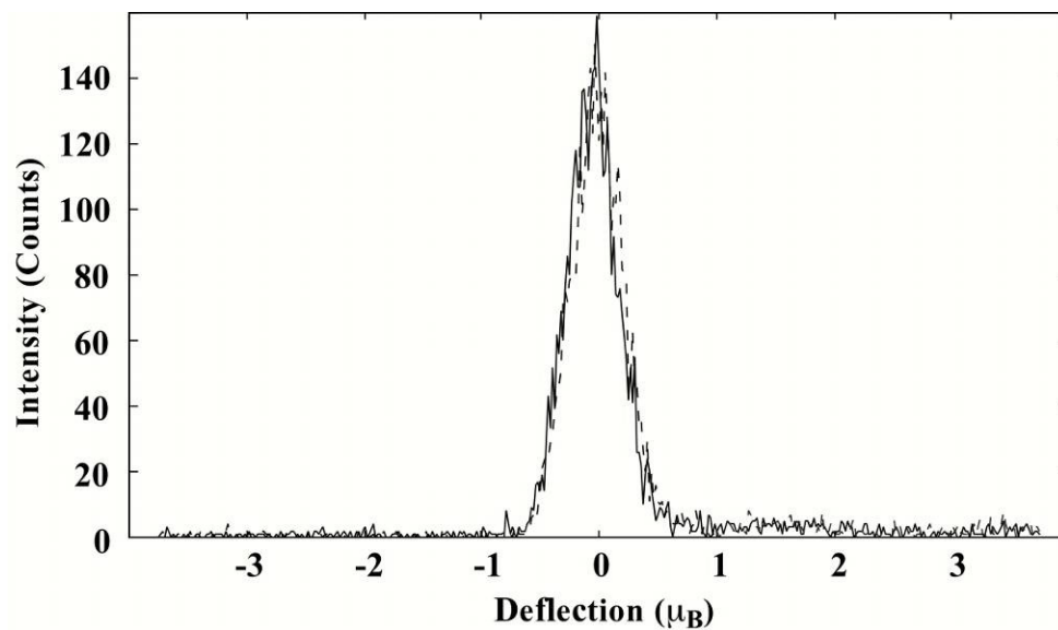
Figure 35: The Stern-Gerlach experiment of Nb_{22} . The dashed line is the peak with zero field and the solid line is after applying 0.9 T. The x-axis scale has been converted to magnetic moment in Bohr magnetons. Almost no visible response to the magnetic field. This is also the case for all even-clusters studied, with the only exception of the dimer.
