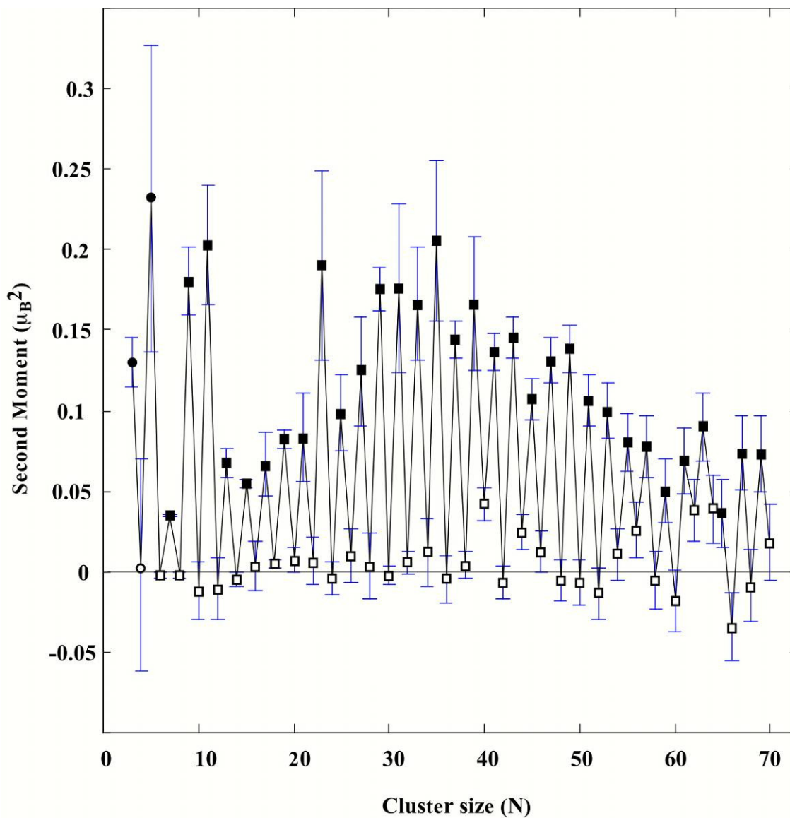
Figure 39: Second moment of the distribution of magnetic moments of niobium clusters. Experiments done at T=20 K for the range Nb_{6-70} (squares) and at T=33 K for Nb_{3-5} (circles). Filled symbols are odd clusters, open symbols are even clusters.
