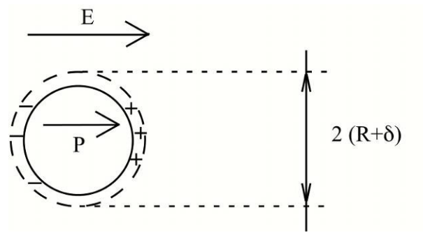
Figure 3: A simple metal cluster in an electric field. Schematic that shows the electronic spill-out effect.
