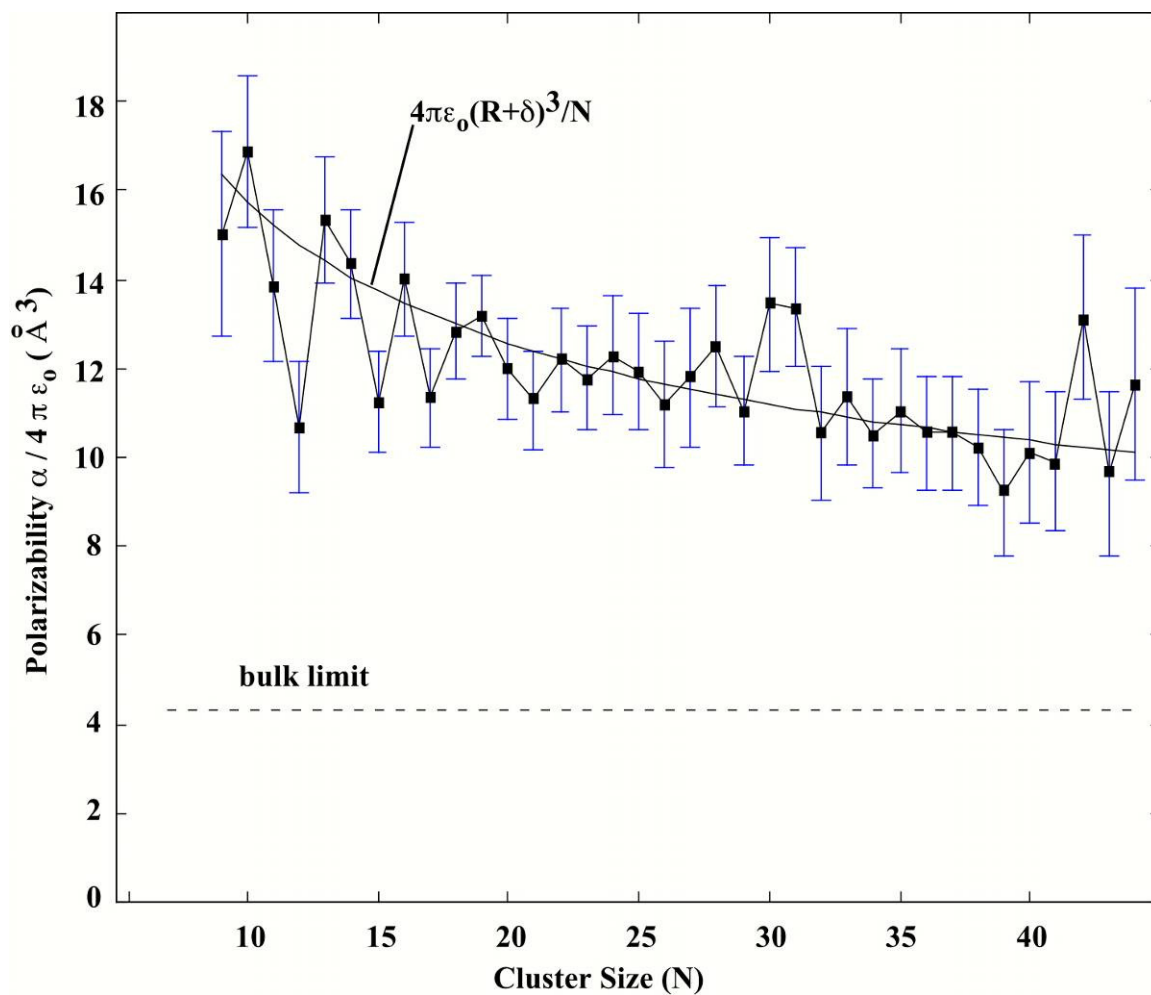
Figure 42: Polarizability per atom of tantalum clusters measured at 300 K and 72 kV/cm. The dashed line is the bulk limit and also shown is a fitting with the spill-out approximation (equation 6) with \delta = 0.19 nm.
